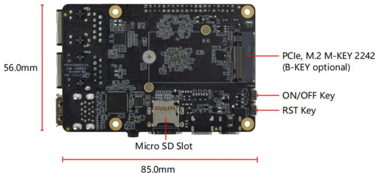
Figure 3 Back View of the DEBIX R3576-01
